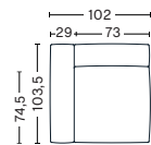
Left armrest Art. S1062 W73/102 x D74,5/103,5 x H37/67 cm Armrest W29 x H67 cm
