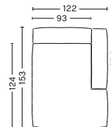
Right armrest Art. S7261 W93/122 x D124/153 x H37/67 cm Armrest W29 x H67 cm
