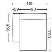
Left armrest Art. S8262 W90/119 x D106,5/135,5 x H37/67 cm Armrest W29 x H67 cm
