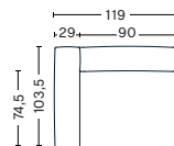
Left armrest Art. S1962 W90/119 x D74,5/103,5 x H37/67 cm Armrest W29 x H67 cm
