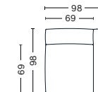
Right corner Art. S1861 W69/98 x D69/98 x H37/67 cm Armrest W29 x H67 cm
