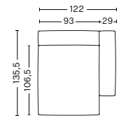
Right armrest Art. S8261 W90/119 x D106,5/135,5 x H37/67 cm Armrest W29 x H67 cm
