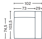
Right armrest Art. S1061 W73/102 x D74,5/103,5 x H37/67 cm Armrest W29 x H67 cm
