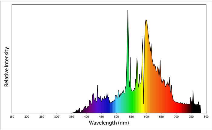
CMH 35W 3000K spectral distribution
