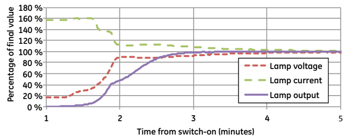
70W CMH-AR111 typical warm-up characteristic
