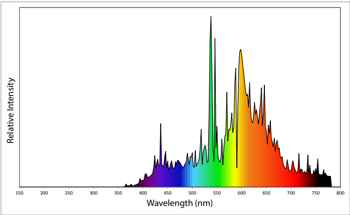
CMH 70W 3000K spectral distribution
