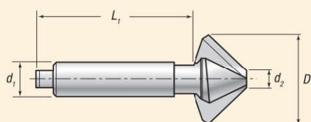
Dimensionstabell
