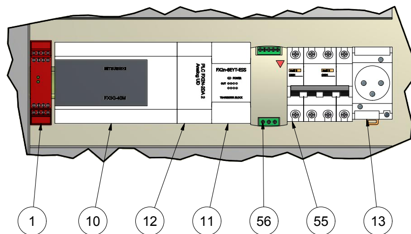
B (1:3)
