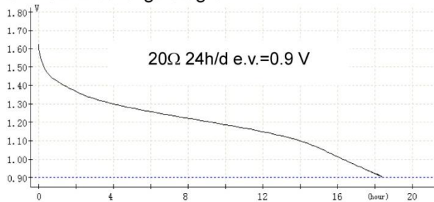
Chart 1. Discharge diagram
