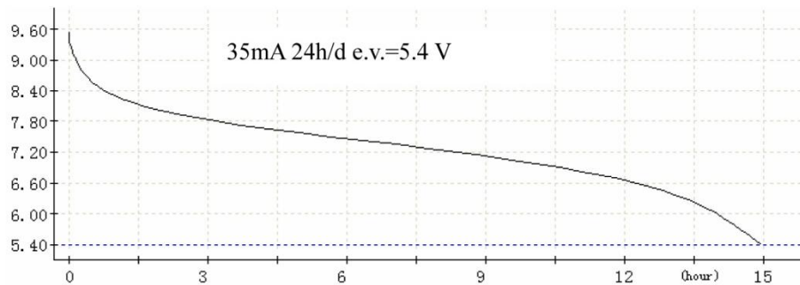
Chart 1. Discharge diagram
