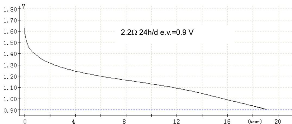
Chart 1. Discharge diagram
