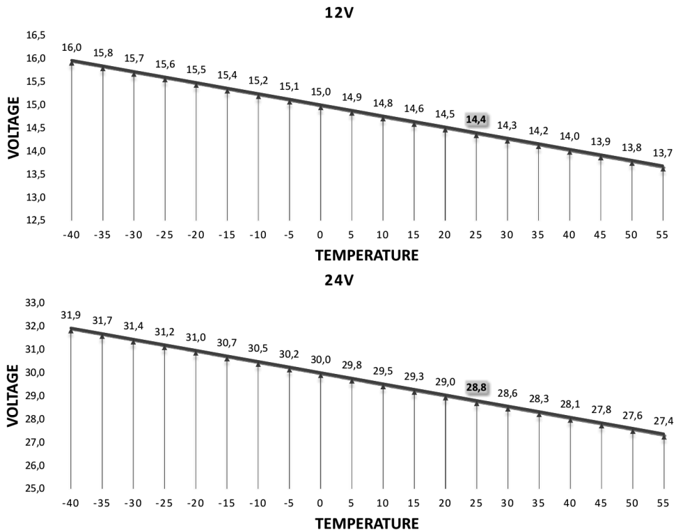
Fig. 3 Temperature compensation
