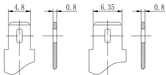
Terminal T1
