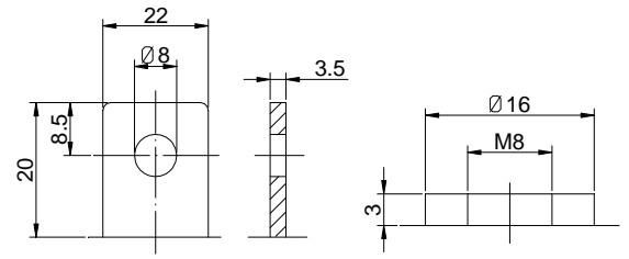
Terminal T5
