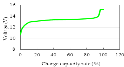
Charge characteristic
