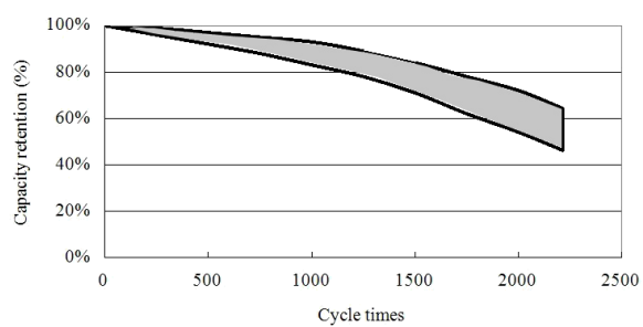
Cycle life
