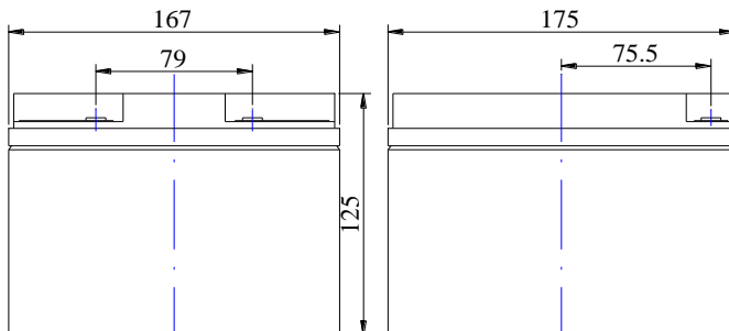
Battery bank spacing required 12.5mm (1/2"inch) minimum
