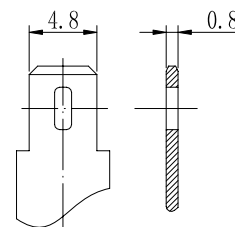
Terminal T1
